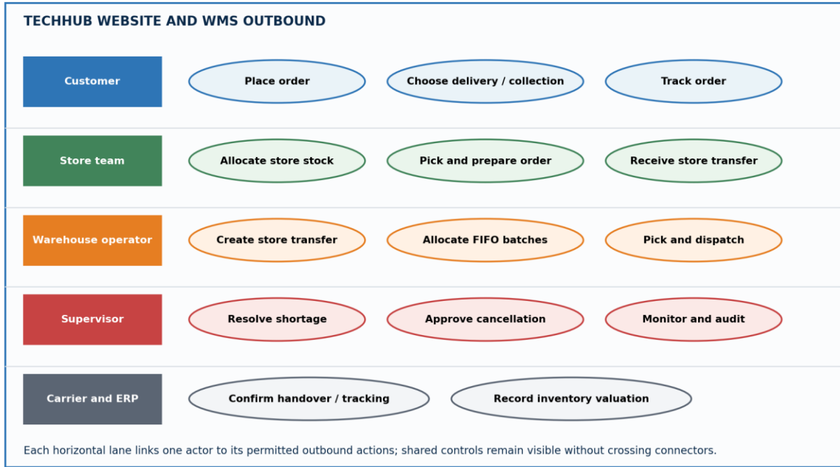
Figure 5. Website and WMS outbound use-case boundary.
