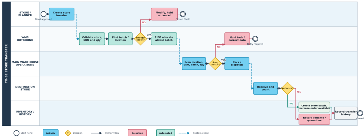
Figure 3B. Target Main Warehouse store-transfer process with FIFO, scan and receipt controls.
